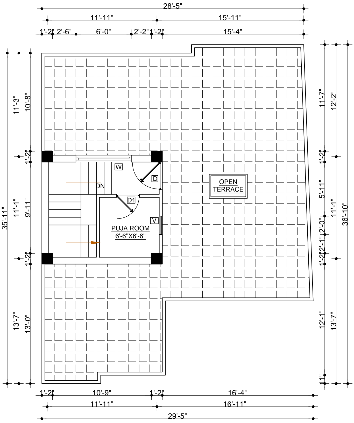
TOP FLOOR PLAN AREA=160.00 SQ.FT.
