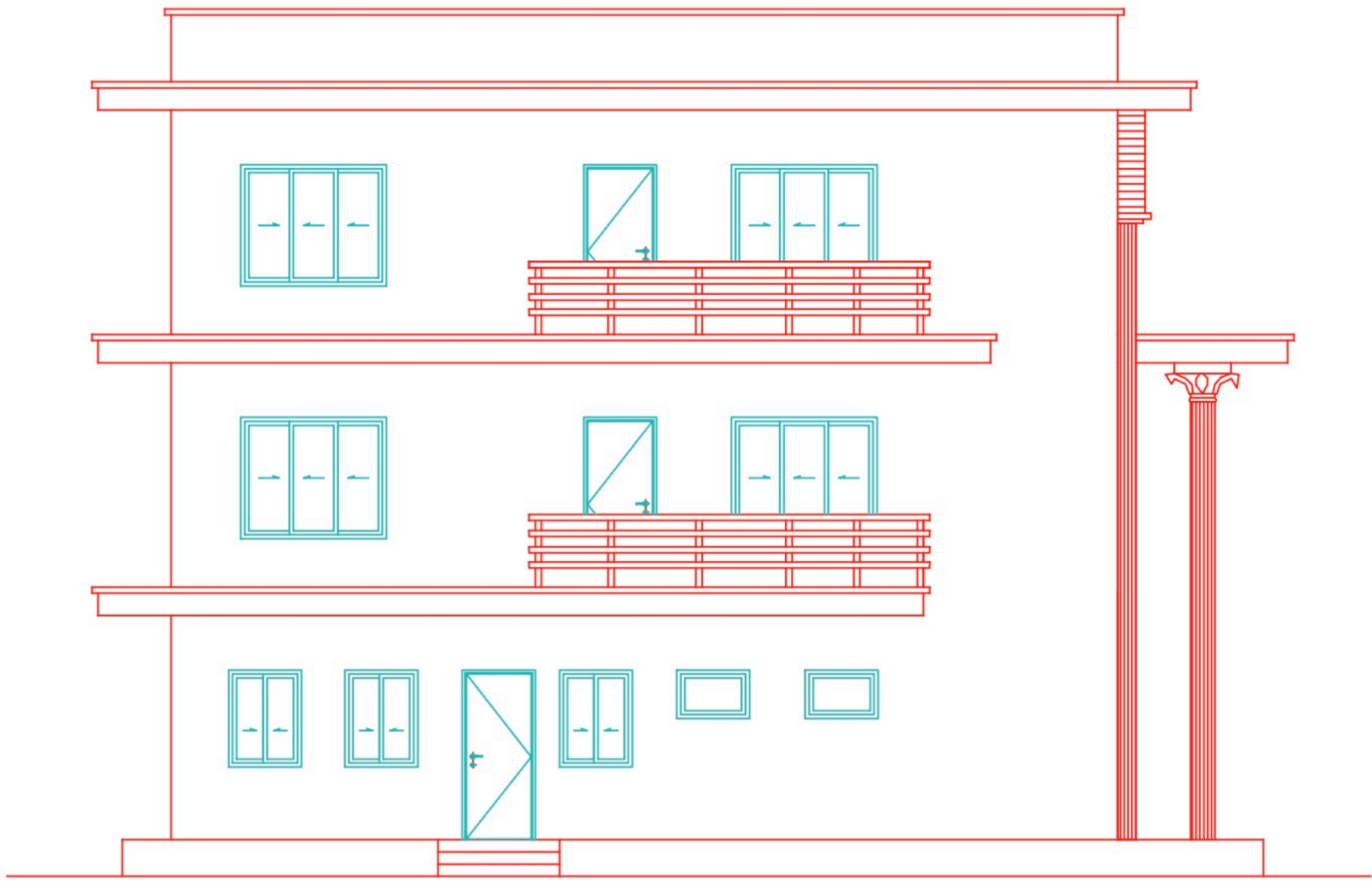
EAST ELEVATION
