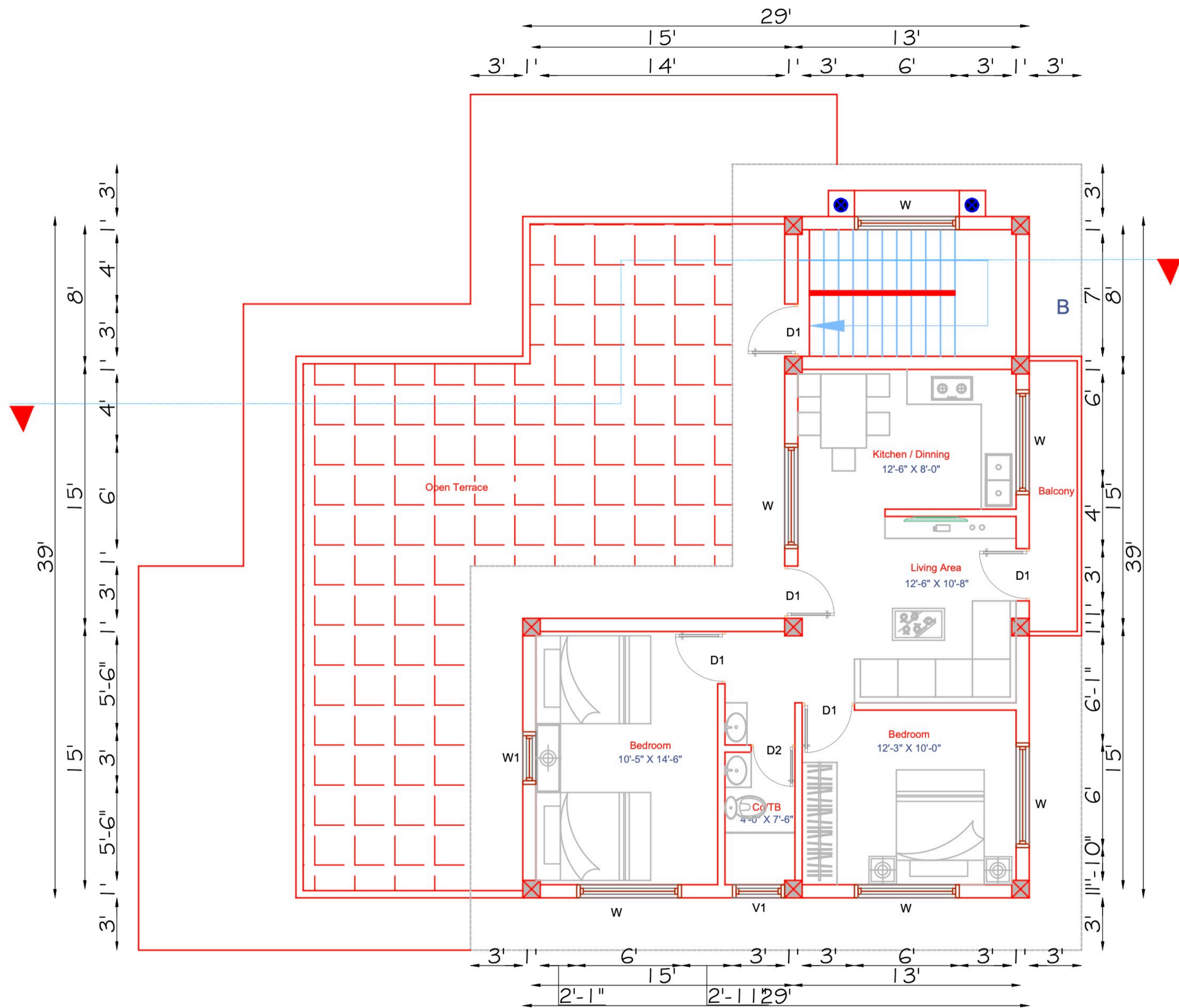
SECOND FLOOR PLAN Built-up Area :786.00 Sq.Ft
