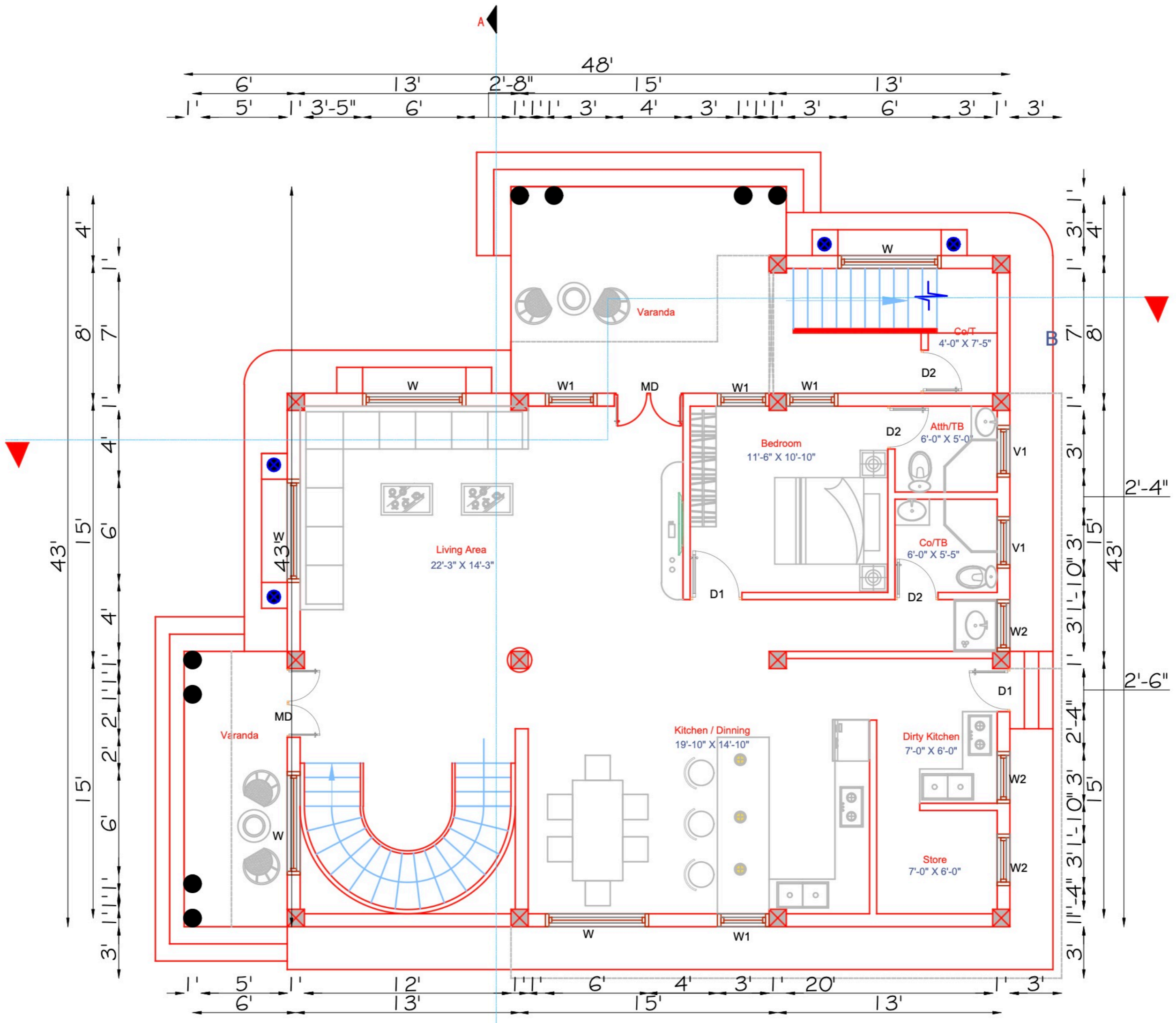
GROUND FLOOR PLAN Plinth Area: 1694.00 Sq.Ft
