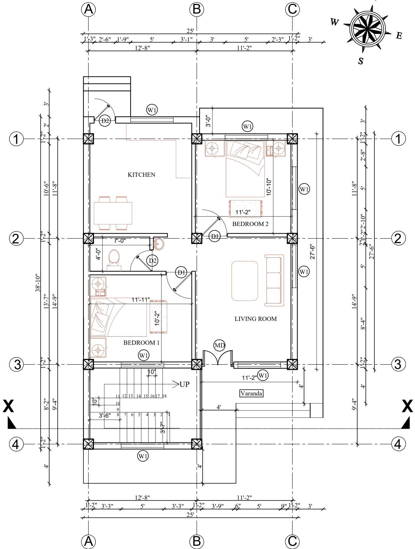
GROUND FLOOR PLAN 841 SQ. FT
