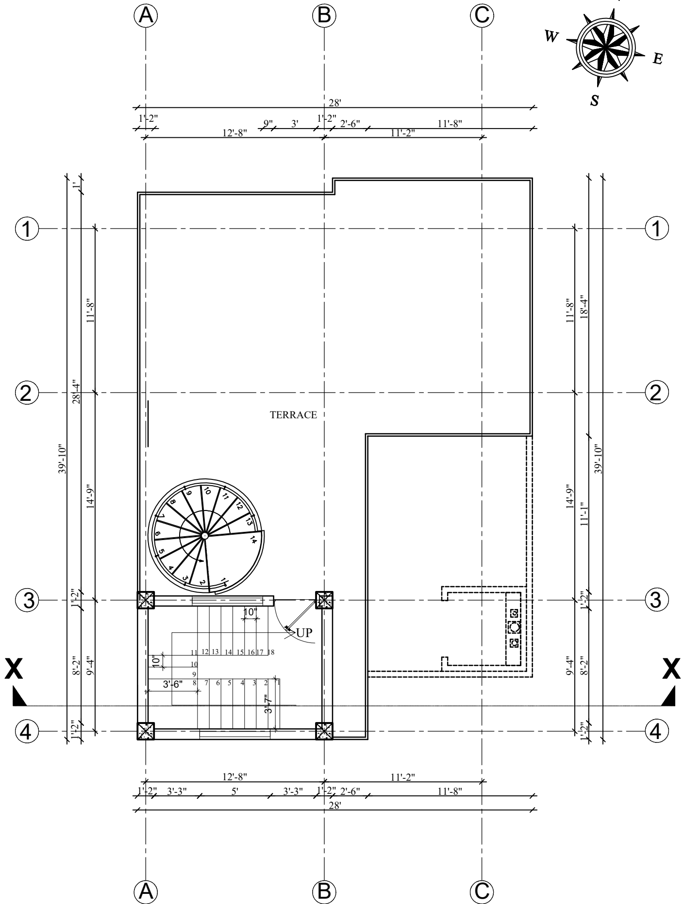
ROOF PLAN 145 SQ. FT
