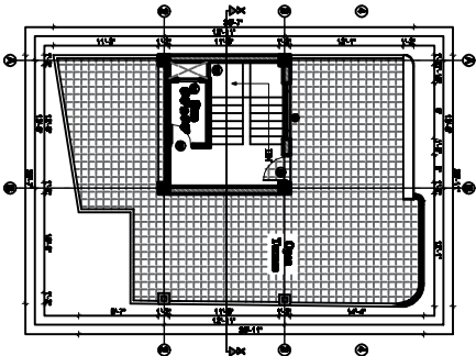
TOP FLOOR PLAN FAR COUNTABLE AREA=800.00 SQ.FT. FAR UNCOUNTABLE AREA(STAIR-COVER)=209.01 SQ.FT. TOTAL AREA=1009.01 SQ.FT.
