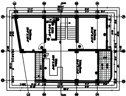
SECOND FLOOR PLAN FAR COUNTABLE AREA=793.77 SQ.FT. FAR UNCOUNTABLE AREA=101.81 SQ.FT. TOTAL AREA=895.58 SQ.FT.
